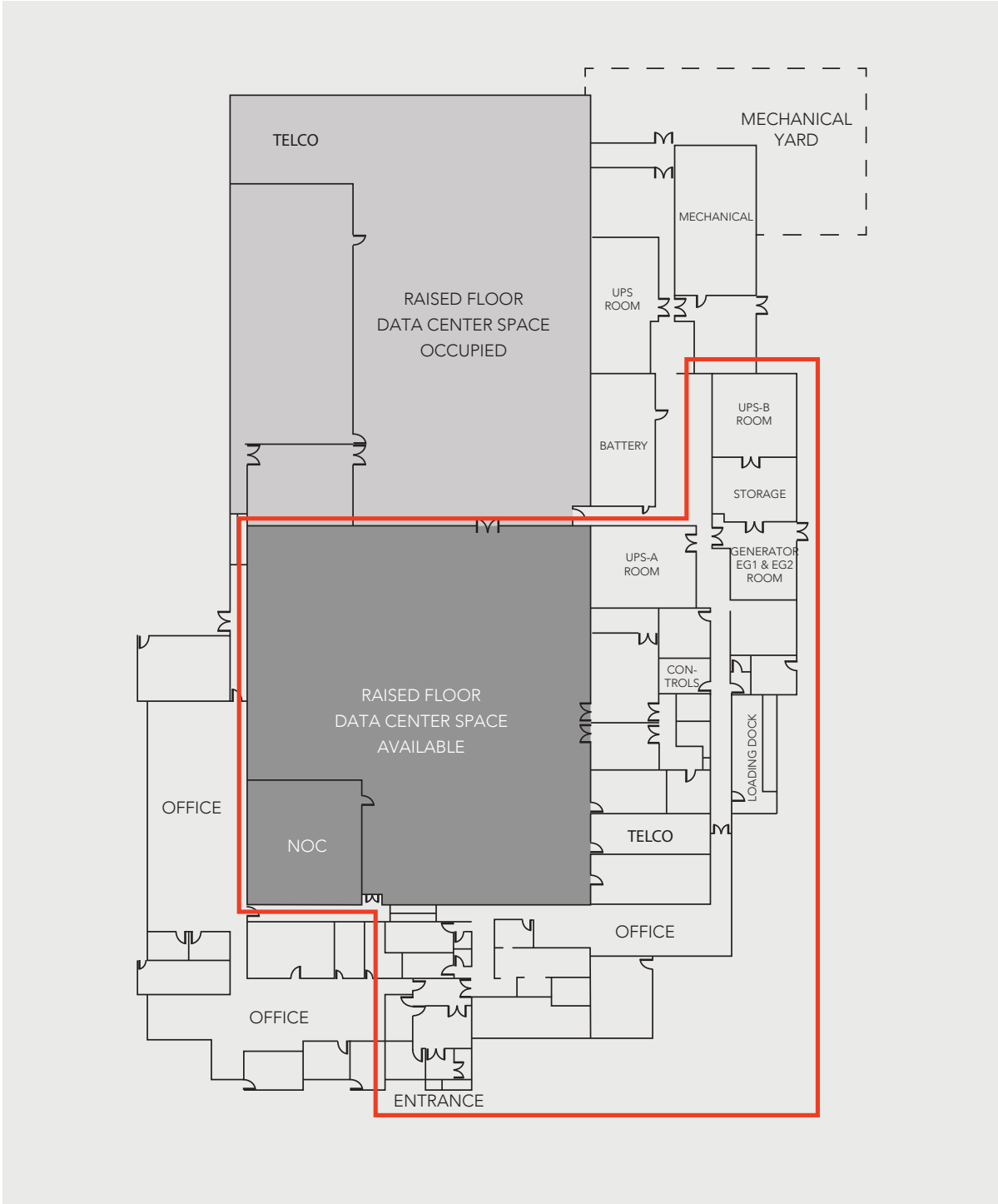
FLOOR PLAN
